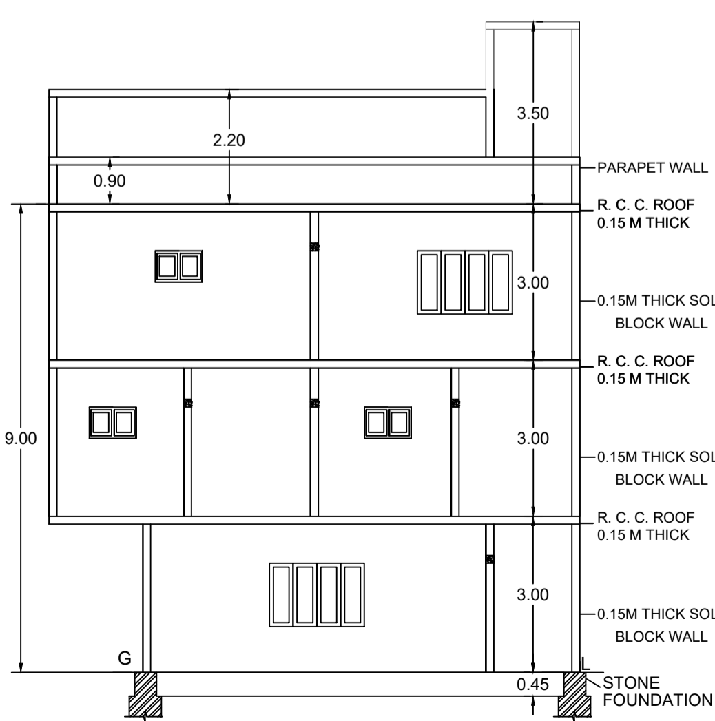
SECTION AT A-A
