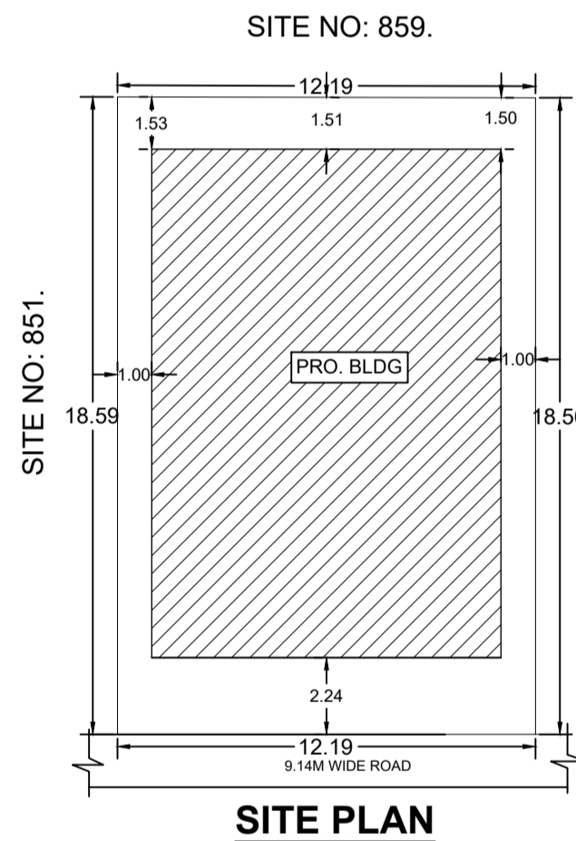
SITE PLAN
